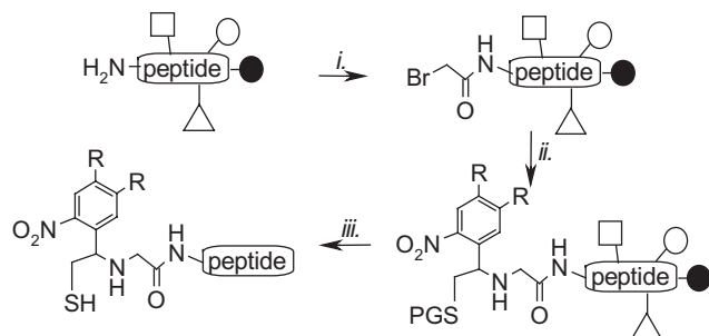
Scheme 4. Introduction of the auxiliary onto a glycine terminal peptide according to the submonomer approach. (i). \text{BrCH}_2\text{COOH} , DIC, DCM; (ii) 9 ( \text{R} = \text{H} ) or 15 ( \text{R} = \text{OCH}_3 ), diea, DMF; (iii) HF or TFA, scavengers. PG = protecting group for thiol functionality.
