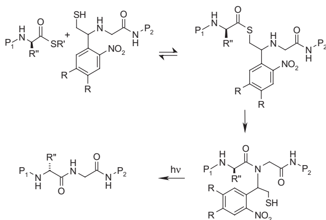
Scheme 1. Peptide ligation mediated by o -nitrobenzyl auxiliaries. P 1 and P 2 : unprotected peptide chains; R = H: auxiliary 9 ; R = OCH 3 : auxiliary 13 ; R' = MPAL; R'' = CH 3 : Ala-Gly junction; R'' = H: Gly-Gly junction.
