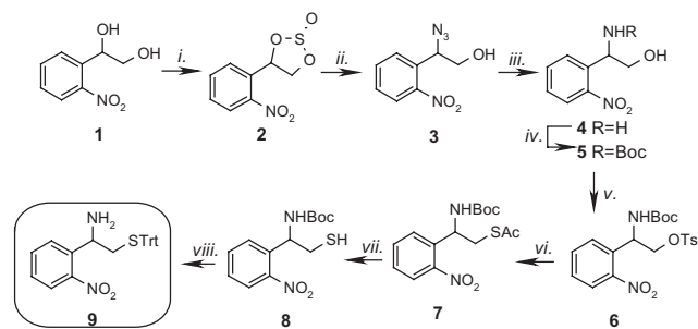
Scheme 2. (i) SOCl 2 , Et 3 N, CH 2 Cl 2 (98%); (ii) NaN 3 , DMF, 60 °C (93%); (iii) PPh 3 , THF, H 2 O (91%); (iv) Boc 2 O, Et 3 N, MeOH (quant.); (v) TsCl, py (98%); (vi) CsCO 3 , AcSH, DMF (98%); (vii) NH 2 OH, MeOH; (viii) TrtOH, TFA (95%) (overall yield 76%).
