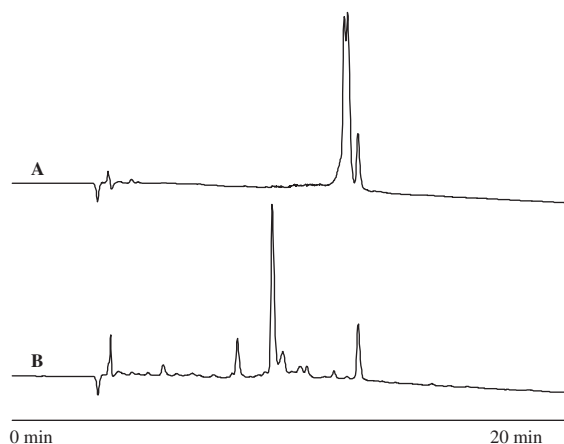
Figure 3. Analytical HPLC trace for the photolysis of purified H -KLAPYRAG-( 9 )-GLLRPFYRK-NH 2 . (A) t = 0 ; (B) t = 20 min. Analytical HPLC conditions: Waters Symmetry 300 C18 column (5 \mu m, 4.6 \times 250 mm); 20–50% B in A linear gradient for 20 min (1 cm 3 /min, 214 nm UV monitor detection) (A = 0.1% aq TFA; B = 0.1% TFA in CH 3 CN).
