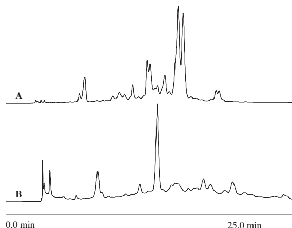
Figure 4. Analytical HPLC trace of photolysis of crude H -LWAPY-RAG-(9)-GLLRPFHRK-NH 2 after 16 h of ligation (A) and of crude H -LWAPYRAGGLLRPFHRK-NH 2 after 20 min of irradiation (B). Analytical HPLC conditions: Waters Symmetry 300 C18 column (5 \mu m, 4.6 \times 250 mm); 20–35% B in A linear gradient for 20 min (1 cm 3 /min, 214 nm UV monitor detection) (A = 0.1% aq TFA; B = 0.1% TFA in CH 3 CN).
