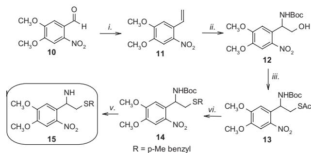
Scheme 3. (i) sodium hexamethyldisilazide, Ph 3 PCH 2 Br, THF (65%); (ii) K 2 OsO 2 (OH) 4 , (DHQD) 2 PHAL, n -prOH, t -Bu carbamate, t -Bu hypochlorite, NaOH, H 2 O (53%); (iii) AcSH, Ph 3 P, DIAD, THF (98%); (iv) MeONa, p -Me benzylbromide (97%); (v) TFA (quant.) (overall yield 32%).
