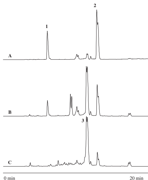
Figure 2. Analytical HPLC trace for the ligation of thioester H -KLAPYRAG-MPAL ( 1 ) with 9 -GLLRPFYRK-NH 2 ( 2 ) to give H -KLAPYRAG-( 9 )-GLLRPFYRK-NH 2 ( 3 ). (A) t = 0 ; (B) t = 60 min; (C) t = 16 h. Analytical HPLC conditions: Waters Symmetry 300 C18 column (5 \mu\text{m} , 4.6 \times 250 mm); 20–50% B in A linear gradient for 20 min (1 \text{cm}^3/\text{min} , 214 nm UV monitor detection) (A = 0.1% aq TFA; B = 0.1% TFA in \text{CH}_3\text{CN} ).
